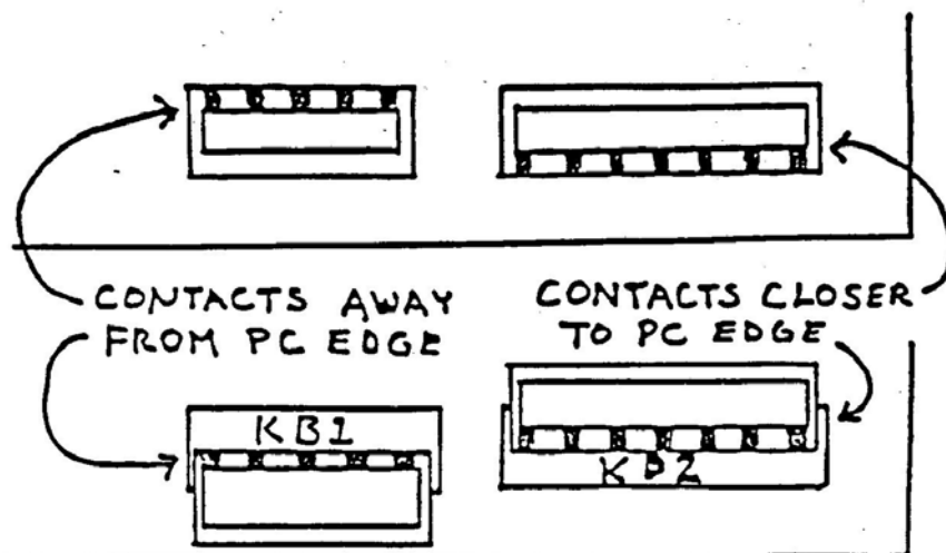
Figure 12b. Properly installed Brand 1 connectors.
